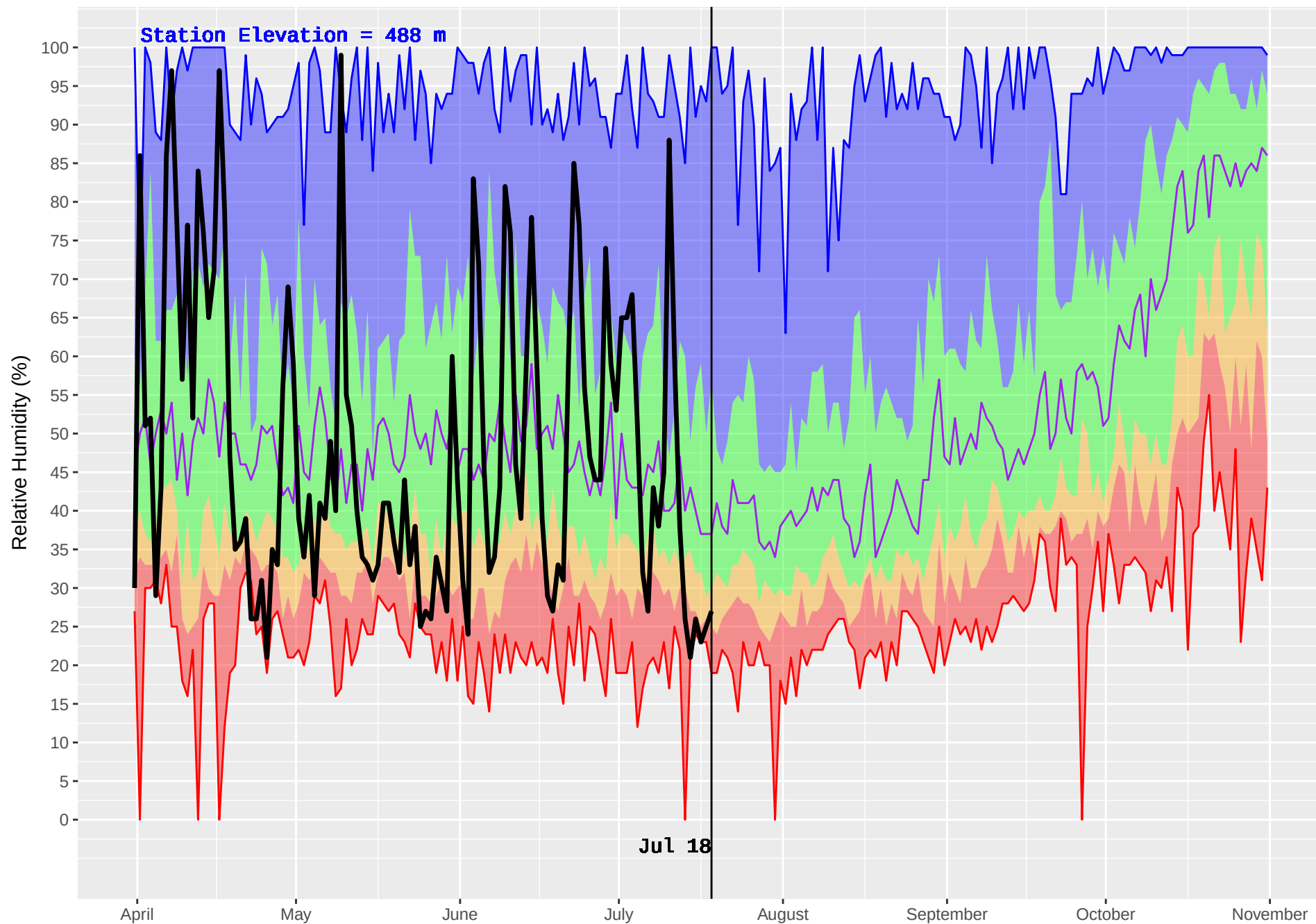
MABEL LAKE 2 (362) : Historical (1987–2016) and Current (2018) Daily Relative Humidity
